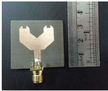
Fig. 2: Fabricated antenna element photograph
