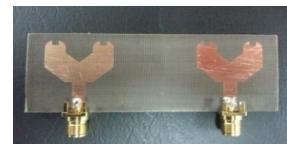
Fig. 6: Fabricated antenna array
