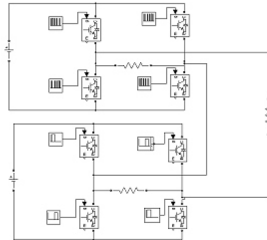
Fig. 6a: Simulation circuit of cascaded nine-level inverter
