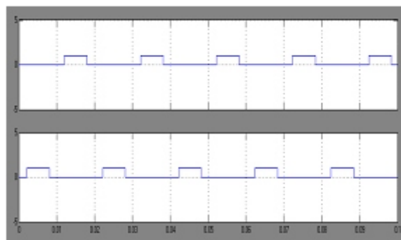
Fig. 6c: Driving pulses for S 5 & S 6
