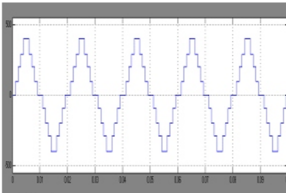
Fig. 6f: Output of nine-level inverter
