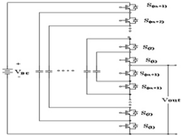
Fig. 4: The m-level capacitor – clamped inverter
