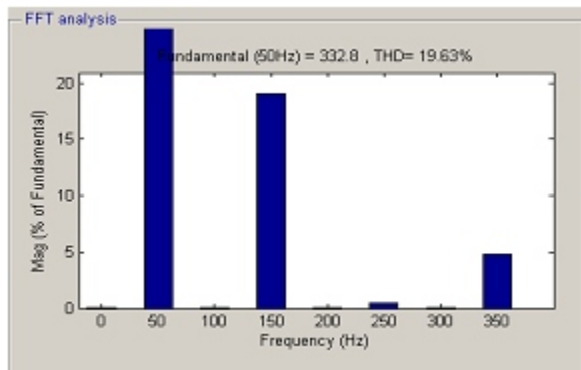
Fig. 6g: Frequency spectrum for output voltage
