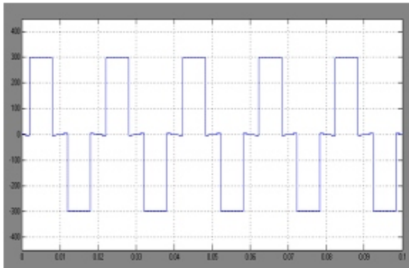
Fig.6e: Output voltage across inverter-2
