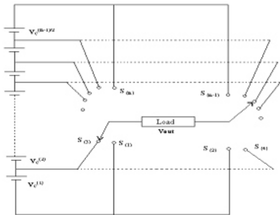
Fig. 5: The m-level inverter using an ‘H’ bridge
