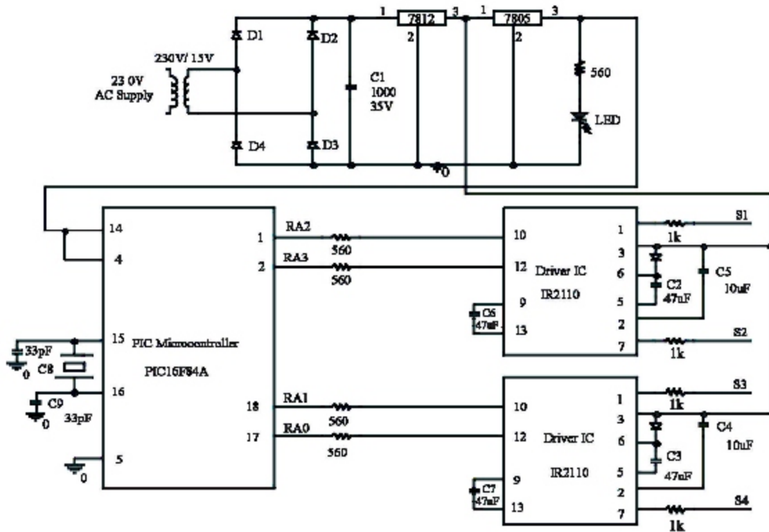
Fig. 7c: Control circuit
